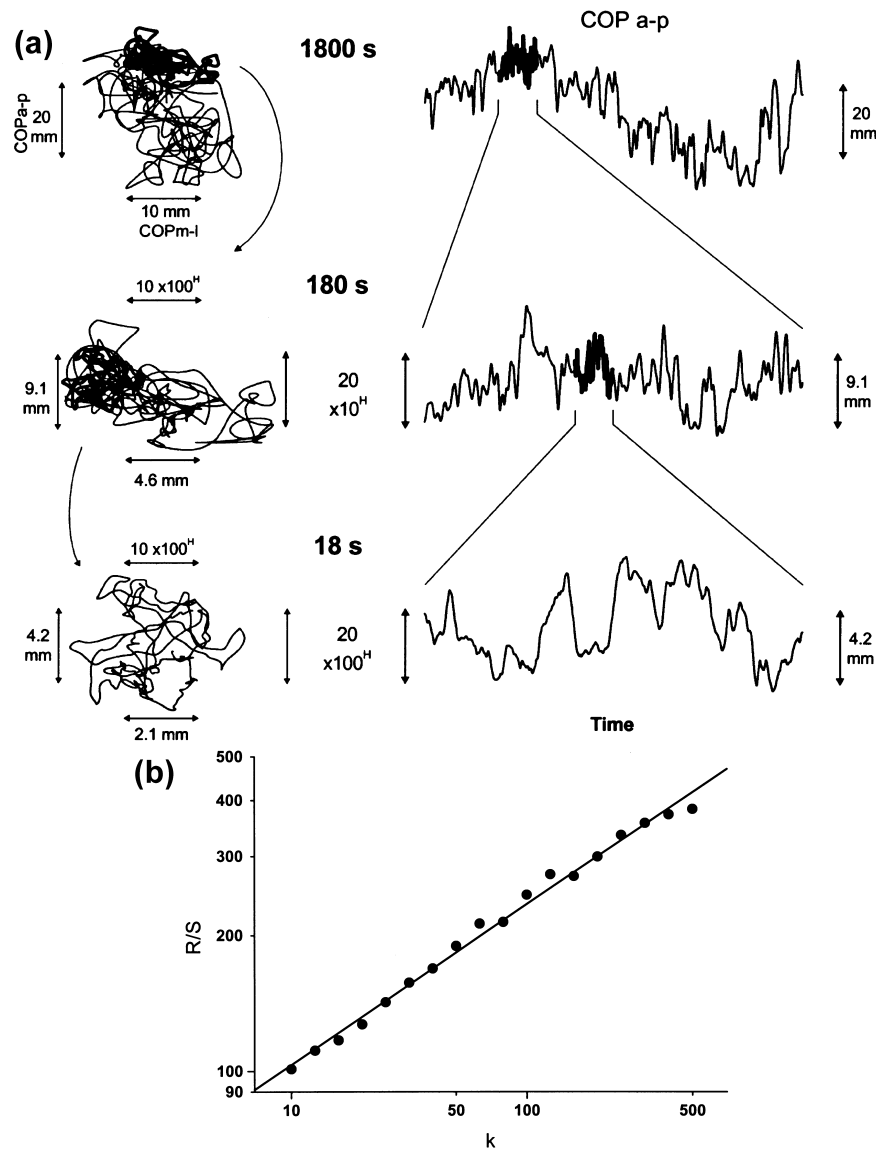
Fig. 1. (a) Stabilograms (left) and anterior-posterior (a-p) COP time series (right) for the entire data during natural standing (1800s, first row), for 1/10 of the data (180 s, second row), and for 1/100 of the data (18 s, third row). The Hurst exponent ( H ) for this example is 0.34, giving a reduction of 2.2 in the amplitude scale for each ten times of reduction of the time scale. Both scaled and real axes are indicated in the 180s and the 18 s plots for illustration. Notice that after each scaling (that is related to the fractal exponent and to the period of time), the three stabilograms and the time series present roughly the same amplitudes in space. For the sake of clarity, not all points are shown for the 1800 and 180 s plots. The difference in the fine structure, observed for the 18-s time series compared to the other two time series, is due to the fact that COP displacements for intervals of up to 1 s display a different behavior [3]. This behavior is most probably due to the inertial characteristics of the body or to the different mechanisms of control of balance (known as open-closed loop model [3]). (b) R/S plot in log-log scale for the 1800-s COP data of the previous example (fit for k = 10 to 600 s, slope = 0.34, r = 0.99 , P < 0.00001 ).
